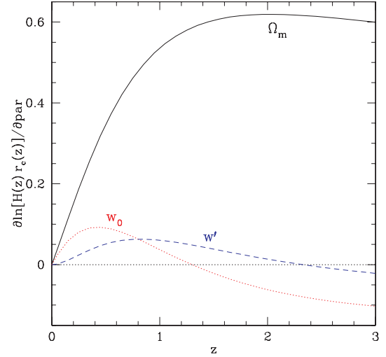
FIG. 3. The sensitivity of the observable, here D = H(z) r_c(z) , to the cosmological parameters is encoded in the derivatives plotted here. The larger the absolute magnitude of the derivative at a particular redshift, the more constraining the observations there.
